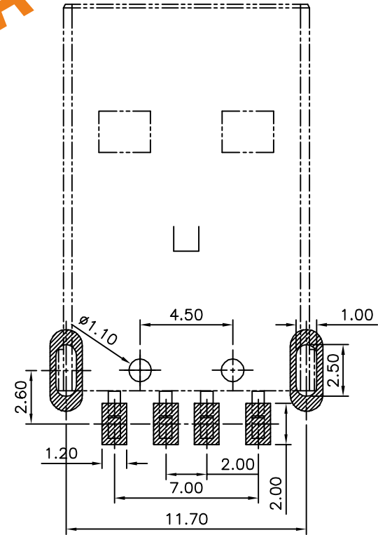
△ Recommended P.C.B. Layout (PCB Board Tolerance ±0.10)
